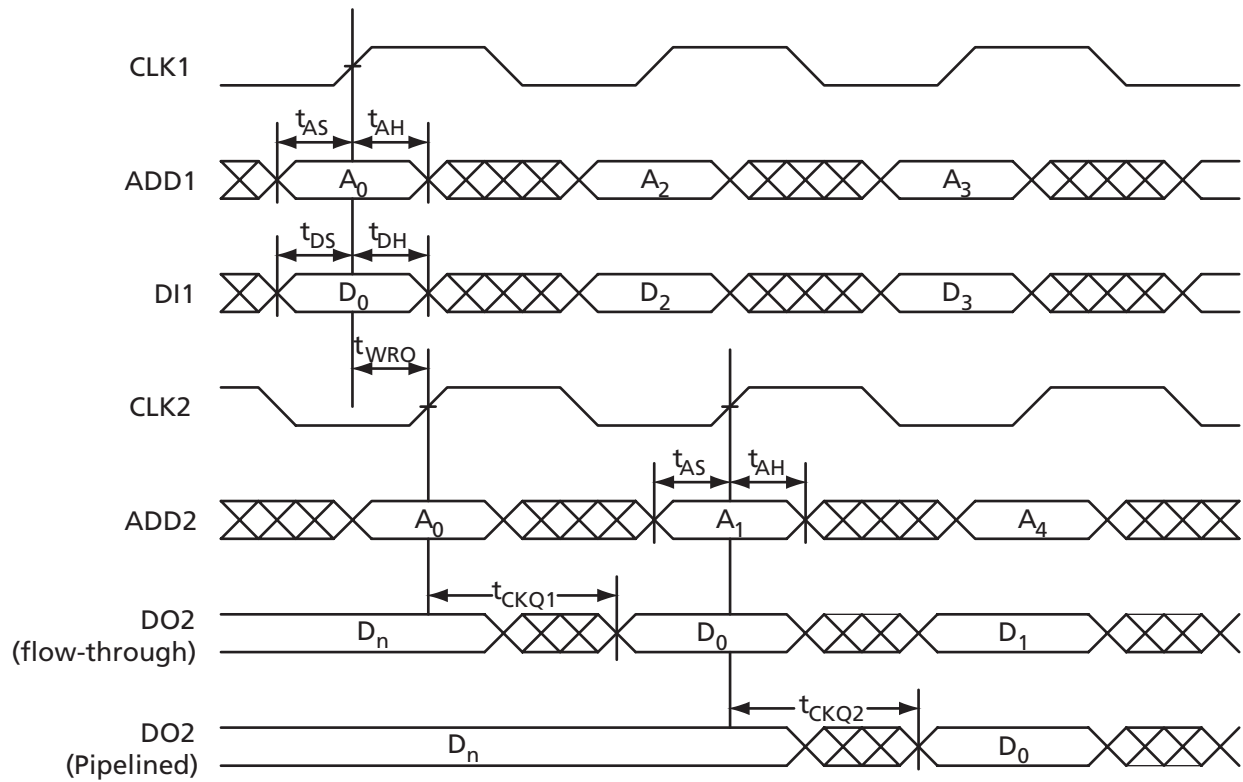
Figure 3-41 • One Port Write/Other Port Read Same
