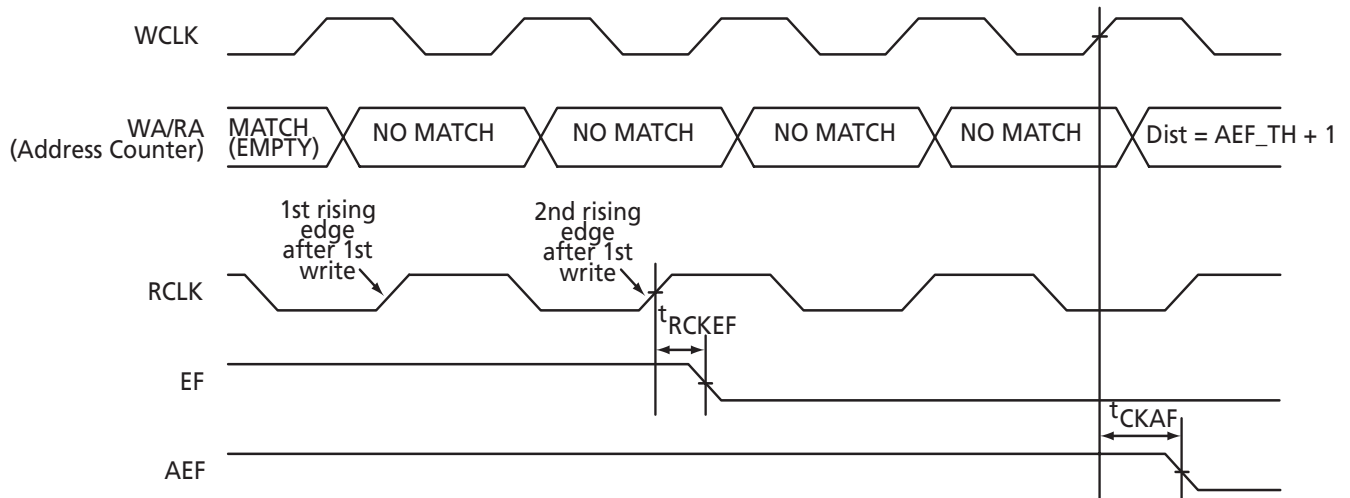
Figure 3-47 • EMPTY Flag and AEMPTY Flag Deassertion
