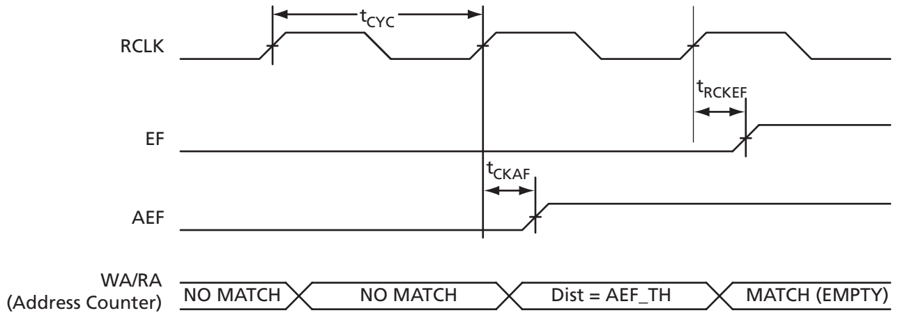
Figure 3-45 • FIFO Reset, EMPTY Flag, and AEMPTY Flag
