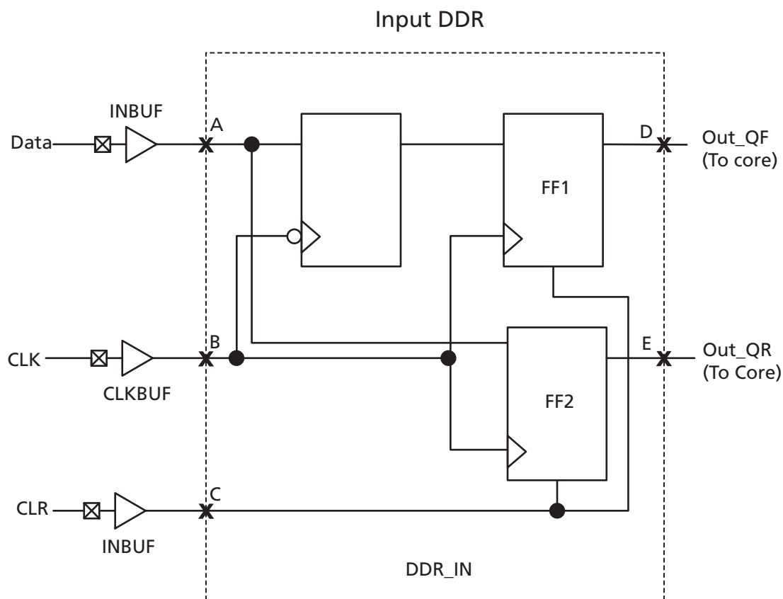
Figure 3-28 • Input DDR Timing Model
