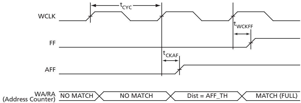
Figure 3-46 • FIFO FULL and AFULL Flag
