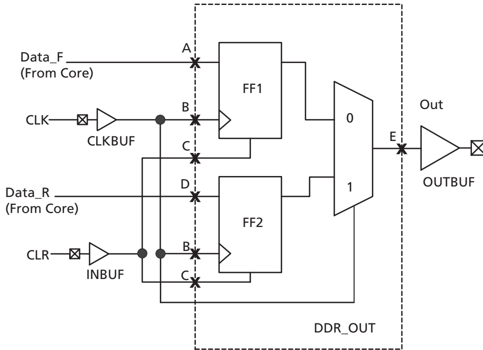
Figure 2-25 • DDR Output Support in ProASIC3E Devices
