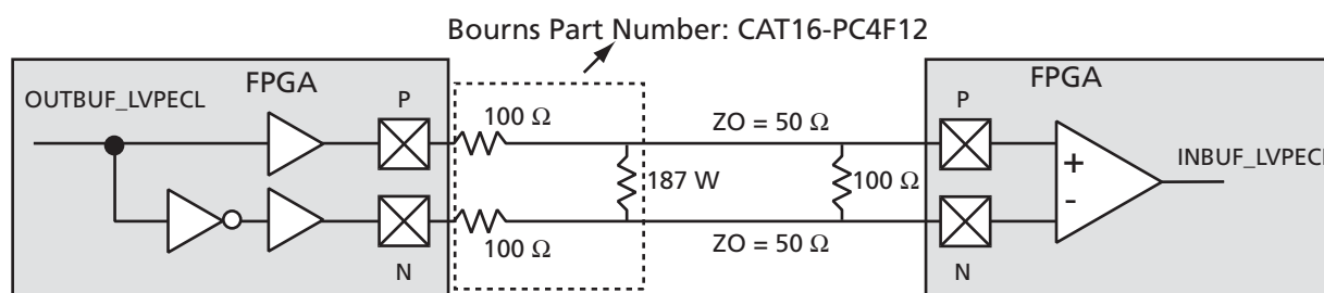
Figure 3-22 • LVPECL Circuit Diagram and Board-Level Implementation
