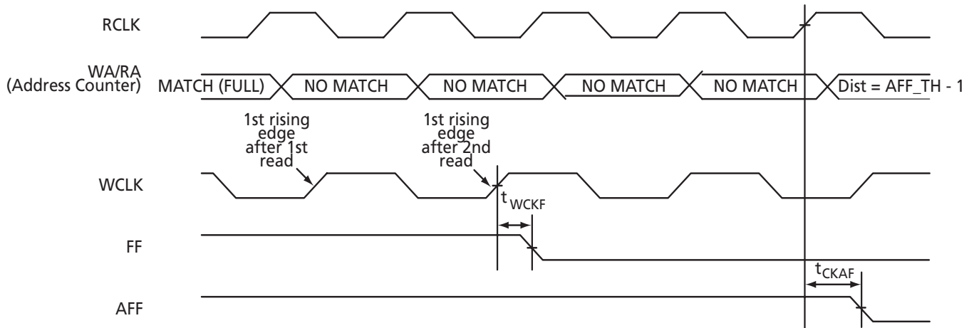
Figure 3-48 • FULL and AFULL Flag Deassertion
