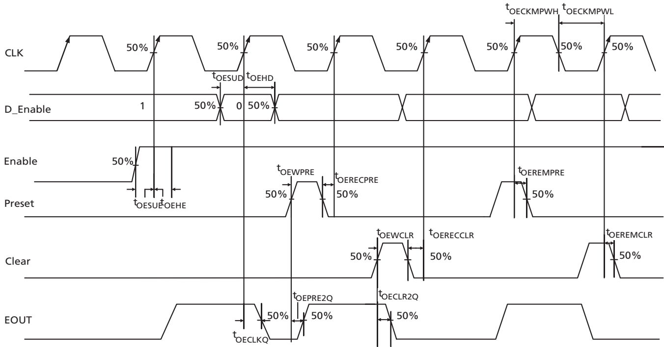
Figure 3-27 • Output Enable Register Timing Diagram
