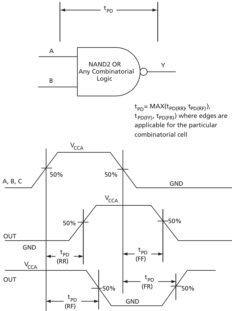
Figure 3-32 • Timing Model and Waveforms
