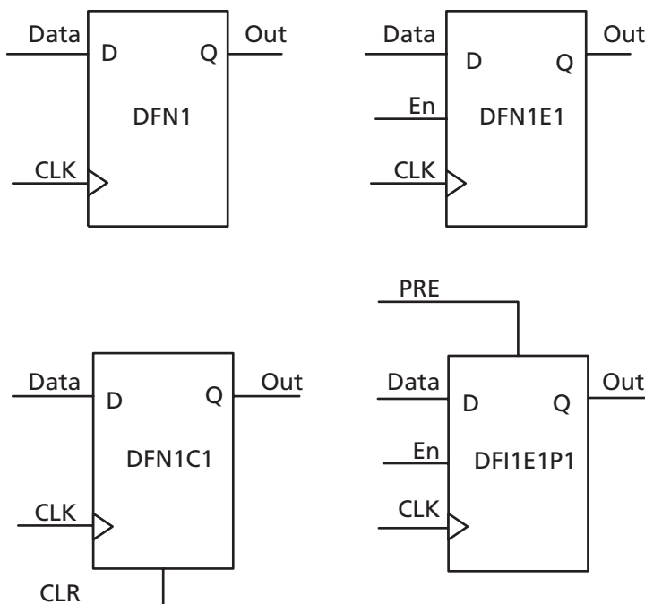
Figure 3-33 • Sample of Sequential Cells
