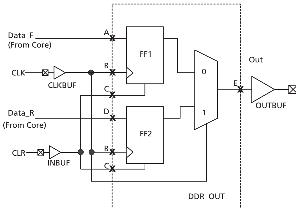
Figure 3-29 • Output DDR Timing Model
