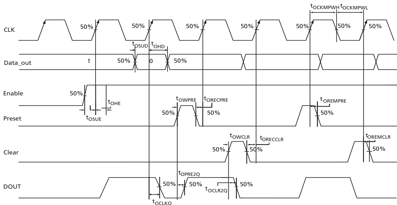
Figure 3-26 • Output Register Timing Diagram
