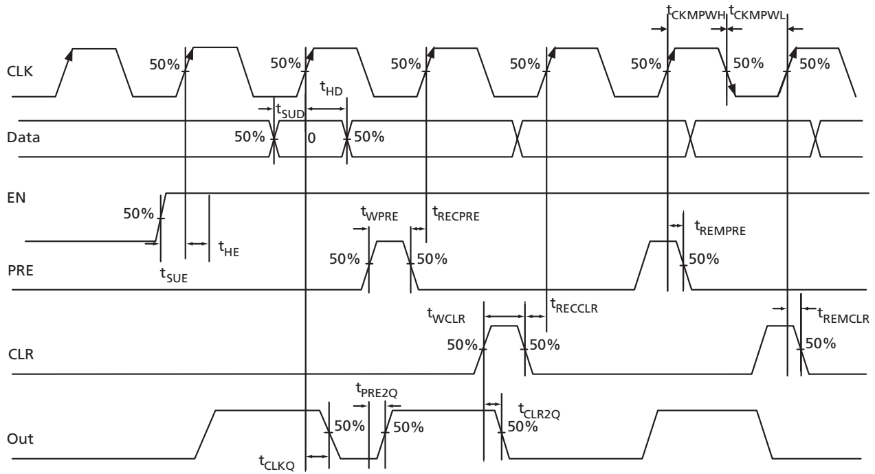
Figure 3-34 • Timing Model and Waveforms
