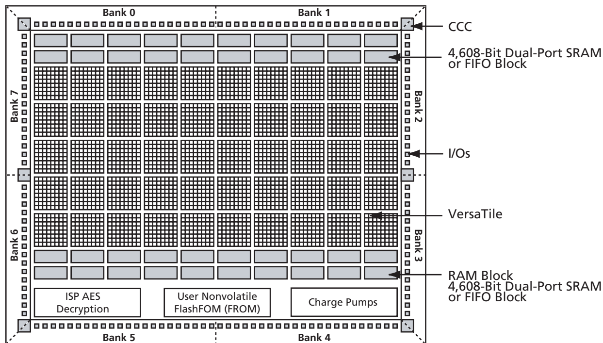
Figure 1-1 • Device Architecture Overview ProASIC3E
