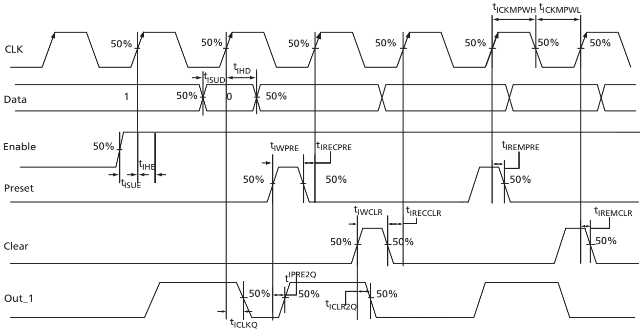
Figure 3-25 • Input Register Timing Diagram
