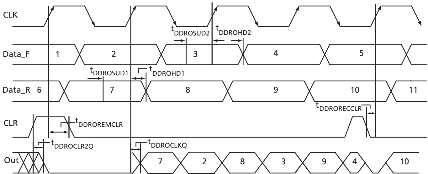
Figure 3-30 • Output DDR Timing Diagram
