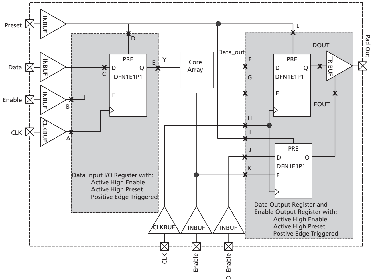
Figure 3-23 • Timing Model of Registered I/O Buffers with Synchronous Enable and Asynchronous Preset
