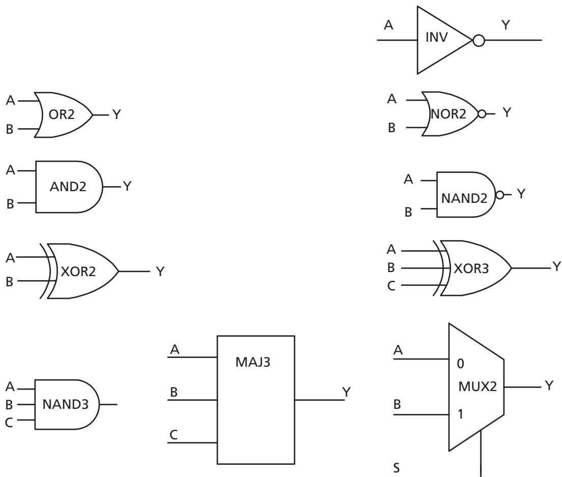
Figure 3-31 • Sample of Combinatorial Cells
