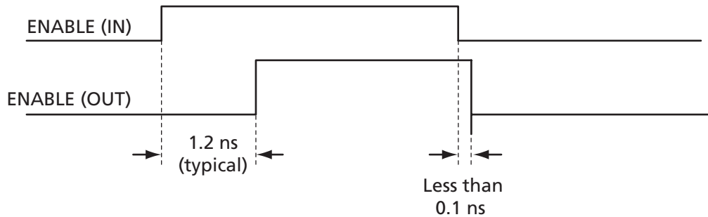
Figure 2-32 • Timing Diagram (Option 2: Enables Skew Circuit)
