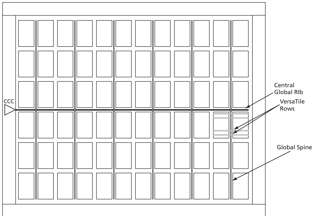
Figure 3-35 • Example of Global Tree Use in an A3PE600 Device for Clock Routing
