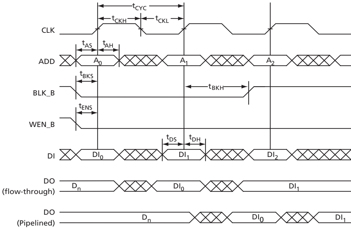
Figure 3-40 • RAM Write, Output as Write Data (WMODE = 1)
