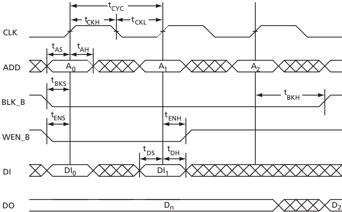
Figure 3-39 • RAM Write, Output Retained (WMODE = 0)
