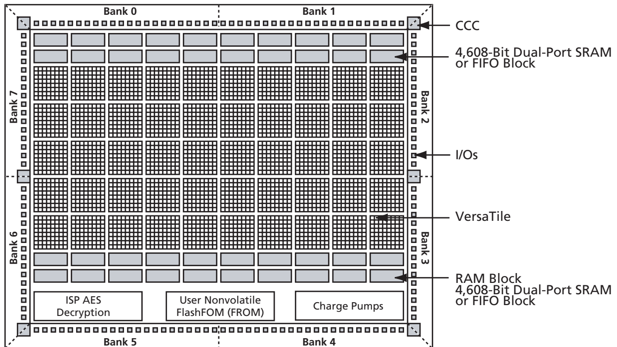
Figure 2-2 • Device Architecture Overview ProASIC3E
