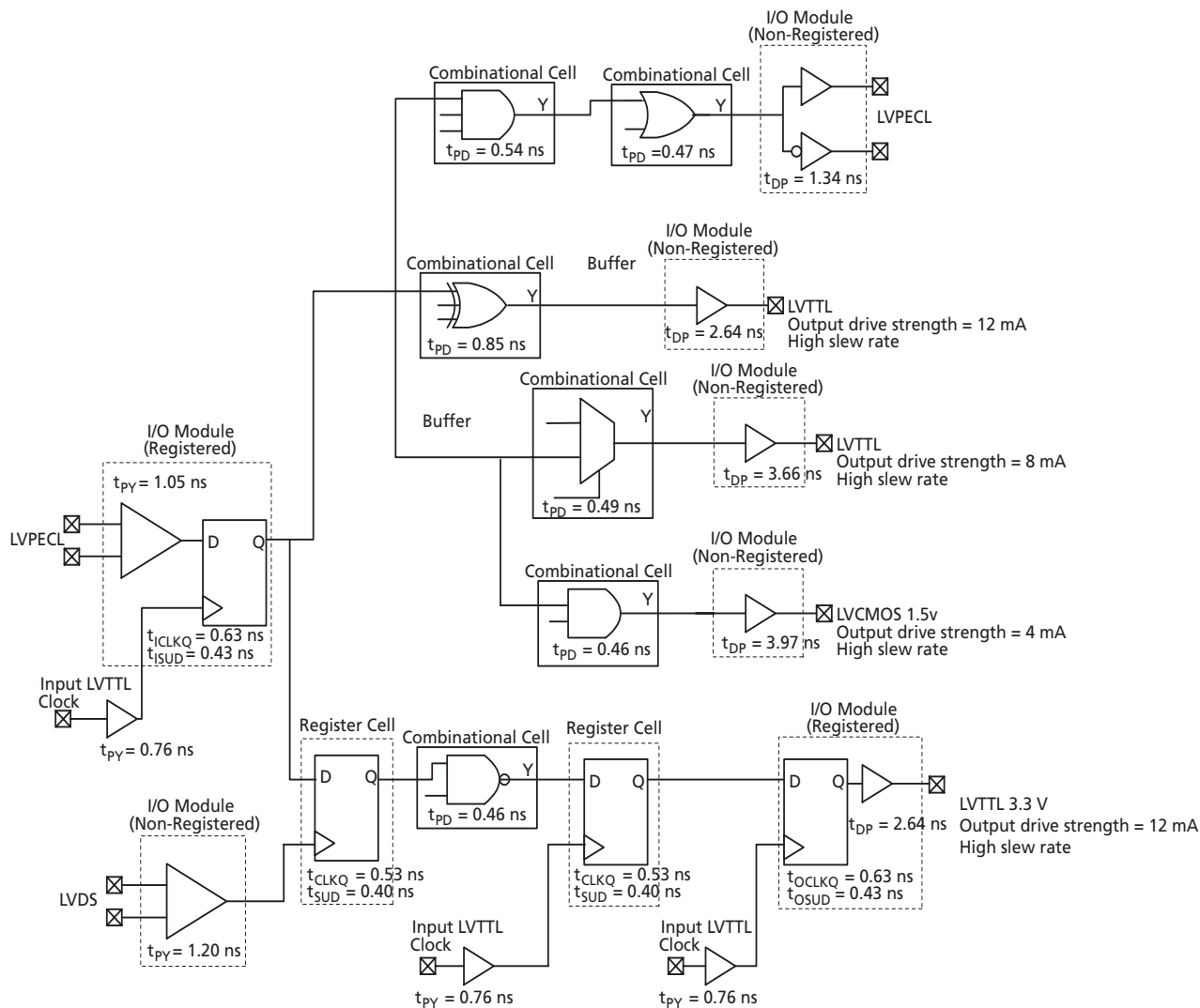
Figure 3-2 • Timing Model
