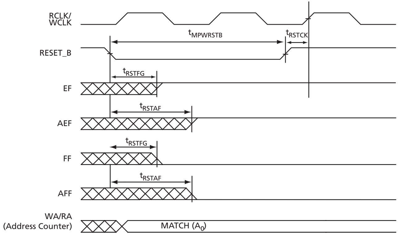
Figure 3-44 • FIFO Reset
