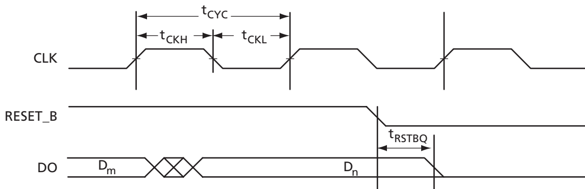
Figure 3-42 • RAM Reset
