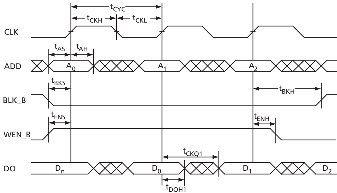
Figure 3-37 • RAM Read for Flow-Through Output
