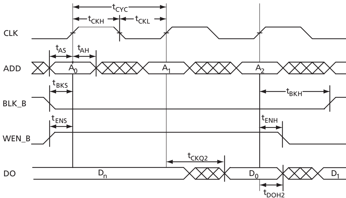
Figure 3-38 • RAM Read for Pipelined Output
